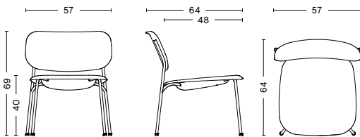
SOFT EDGE 101 | FULL UPHOLSTERY WIDTH 57 CM DEPTH 64 CM HEIGHT 69 CM SEAT HEIGHT 40 CM SEAT DEPTH 48 CM
