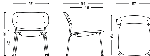
SOFT EDGE 100 | SEAT UPHOLSTERY WIDTH 57 CM DEPTH 64 CM HEIGHT 69 CM SEAT HEIGHT 40 CM SEAT DEPTH 48 CM
