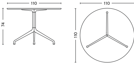
DIAMETER 110 CM HEIGHT 74 CM
