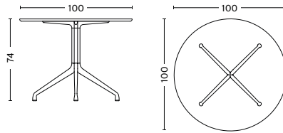
DIAMETER 100 CM HEIGHT 74 CM
