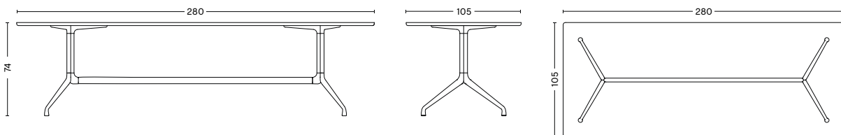
LENGTH 280 CM WIDTH 105 CM HEIGHT 74 CM
