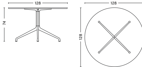
DIAMETER 128 CM HEIGHT 74 CM
