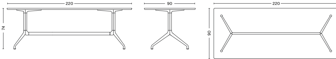
LENGTH 220 CM WIDTH 90 CM HEIGHT 74 CM
