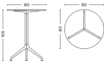
DIAMETER 80 CM HEIGHT 105 CM
