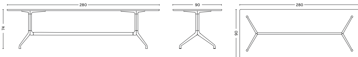
LENGTH 280 CM WIDTH 90 CM HEIGHT 74 CM
