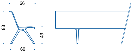
H=83cm | mid backrest
