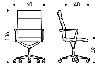
UNA.915GR | swivel chair, fixed height
