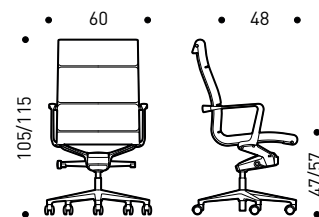
UNA.919T | swivel chair, height adjustable, tilting mechanism
